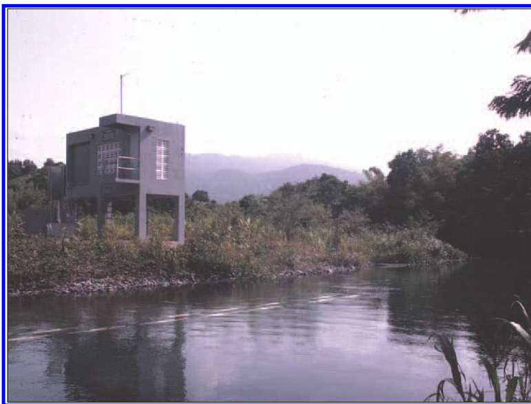
Figure 5. The in-channel withdrawal structure located on the Río Mameyes, Puerto Rico. Water is pumped from the submerged stainless steel risers to the pumphouse on the bank. Photograph: James March.
